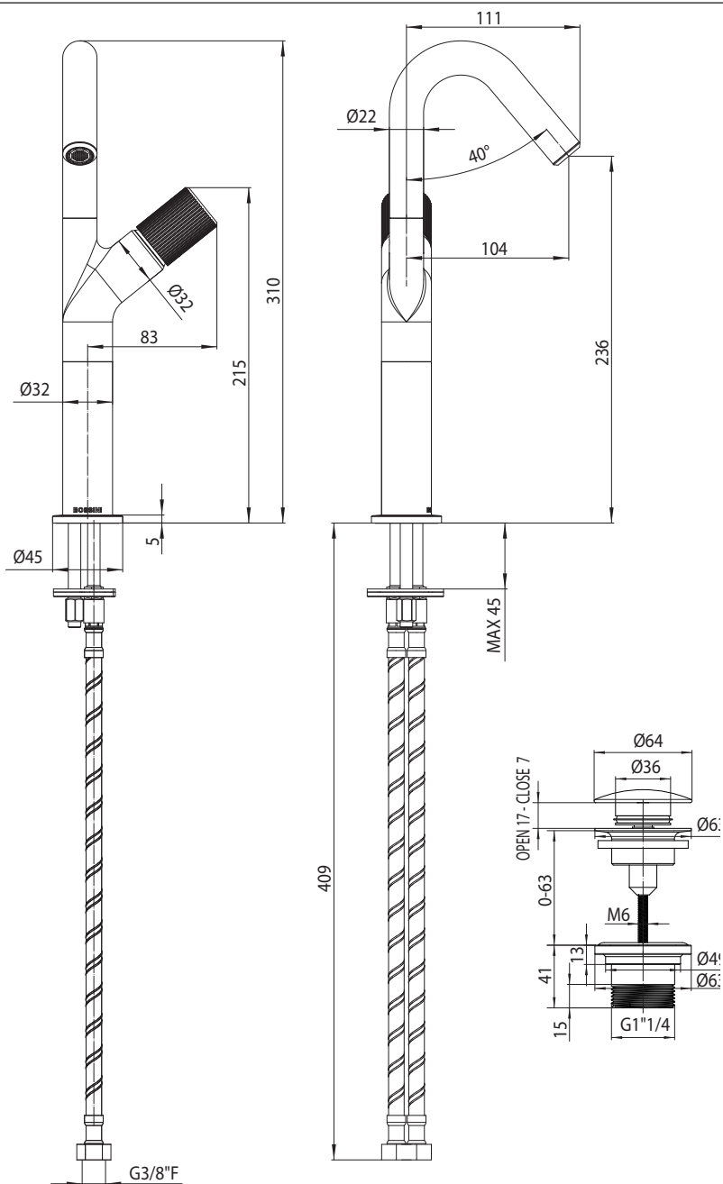
Z00903 - PLY High Basin mixer
