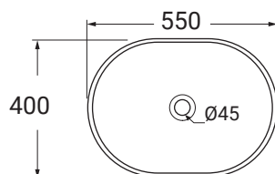
APPOGGIO OVER COUNTER
