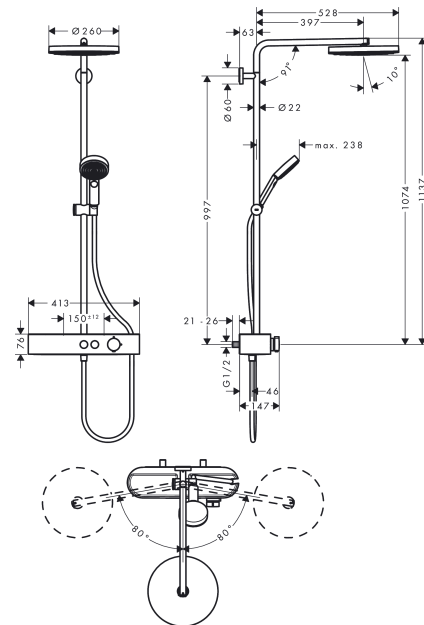
Scale drawing
